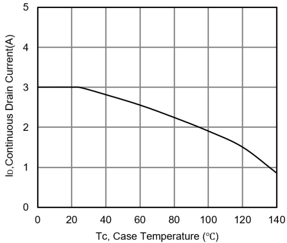
Continuous Drain current vs. Tc
