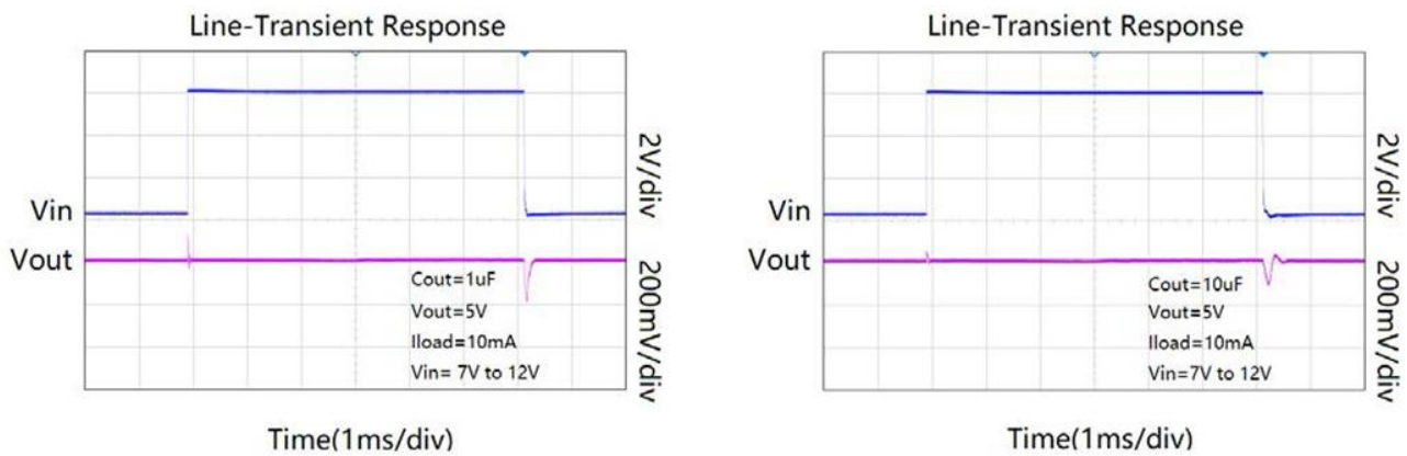
Figure 1. Line-Transient Response
