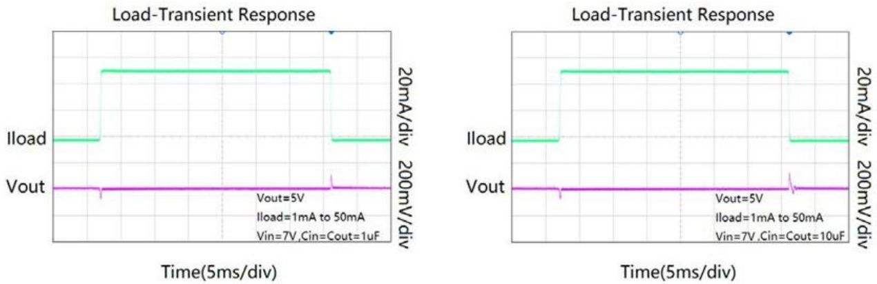
Figure 2. Load-Transient Response
