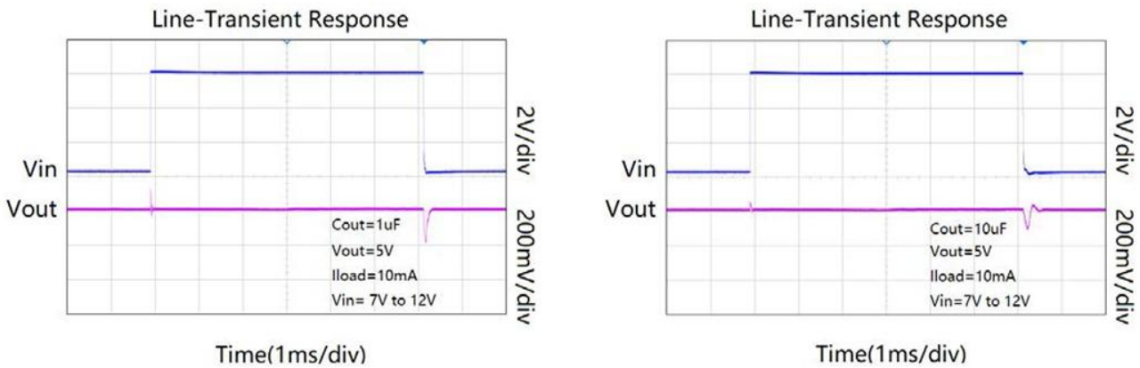
Figure 1. Line-Transient Response
