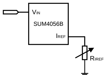
Figure 1. 充电电流设置 1
