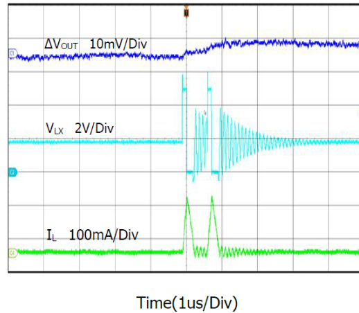
Output Ripple
