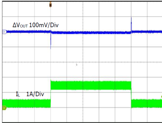
Time(1ms/Div)
