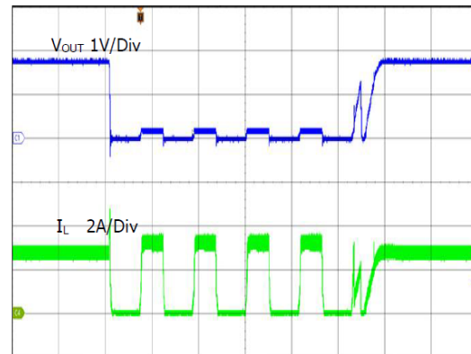
Time(2ms/Div)
