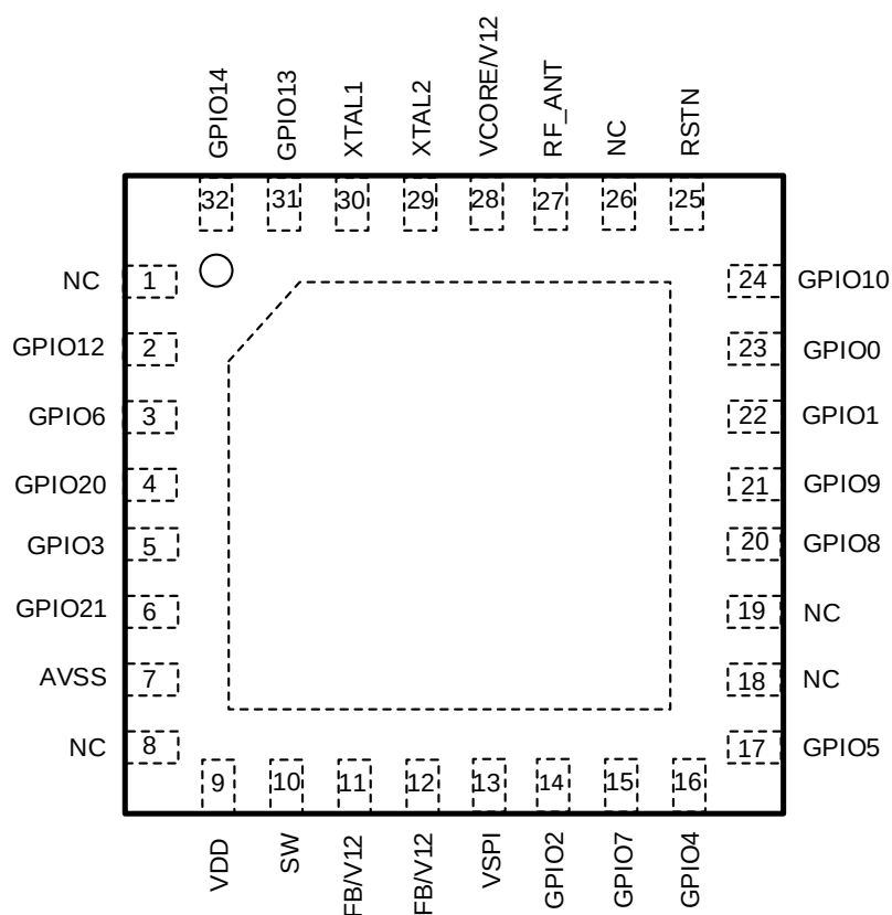
QFN5x5-32
